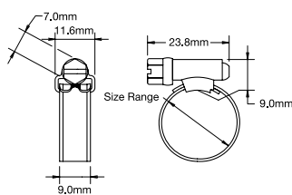
Part No. SMP000 – SMP00
