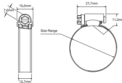
Part No. SMP0A – SMP13
