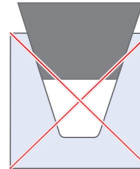
Belt too large / pulley groove too small
